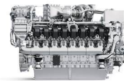
Series 4000 Proven operations reliability in all conditions paired with cutting-edge emissions technology. 1,000-3,300 kW (1,341-4,425 bhp)
