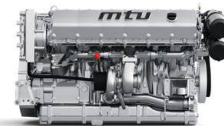
Series 1600 Extremely compact rail engine for smooth operation and extremely low emission values. 565-736 kW (758-987 bhp)
