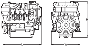
Dimensions: Engines with standard equipment
