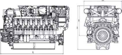
Dimensions: Engines with standard equipment
