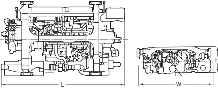
Dimensions: PowerPacks with standard equipment
