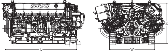
Dimensions: Engines with standard equipment
