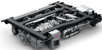
— Horizontally mounted inline engines
