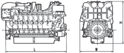
Dimensions: Engines with standard equipment
