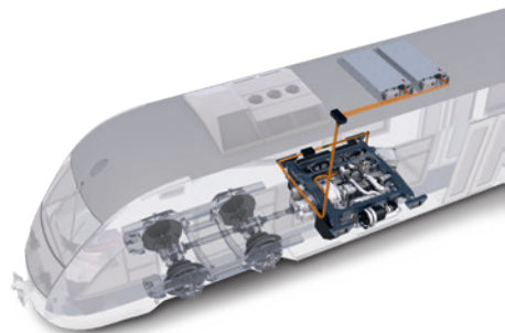
Roof mounting of mtu EnergyPacks
