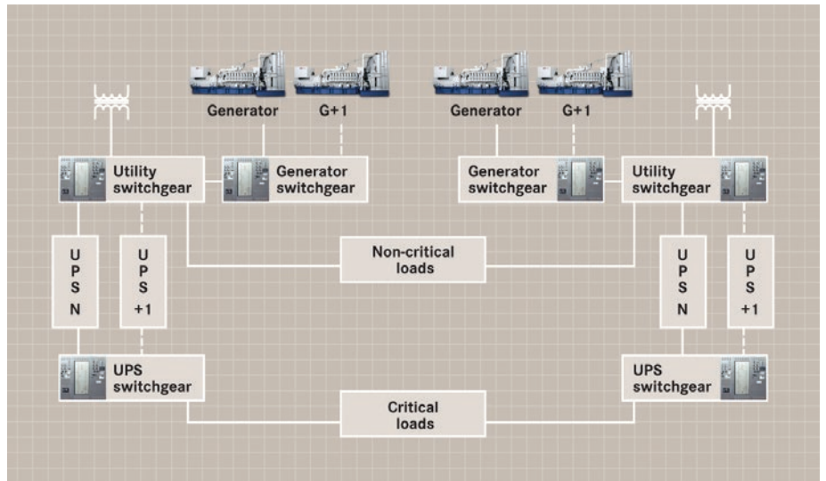
Figure 2. A standby power system with Tier IV design topology and full N+1 redundancy in utility supply, UPS systems and generator sets. This design has been shown to exhibit upwards of 99.99% annual availability.
