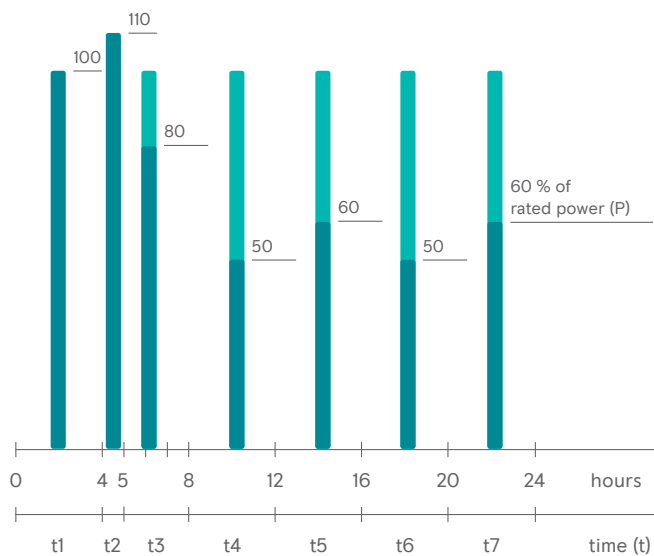
Figure 4. Typical PRP load profile
