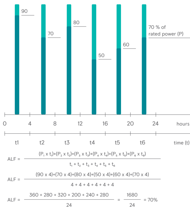
Figure 1. Average load factor
