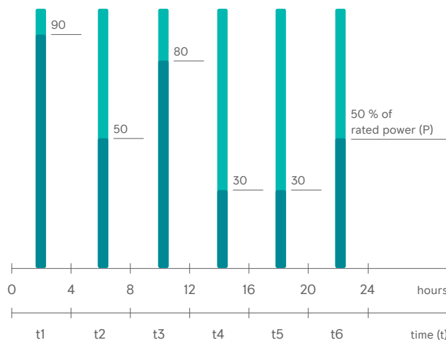
Figure 3. Typical ESP load profile
