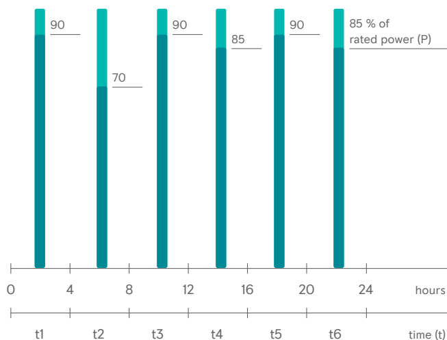
Figure 2. Mission-critical load profile
