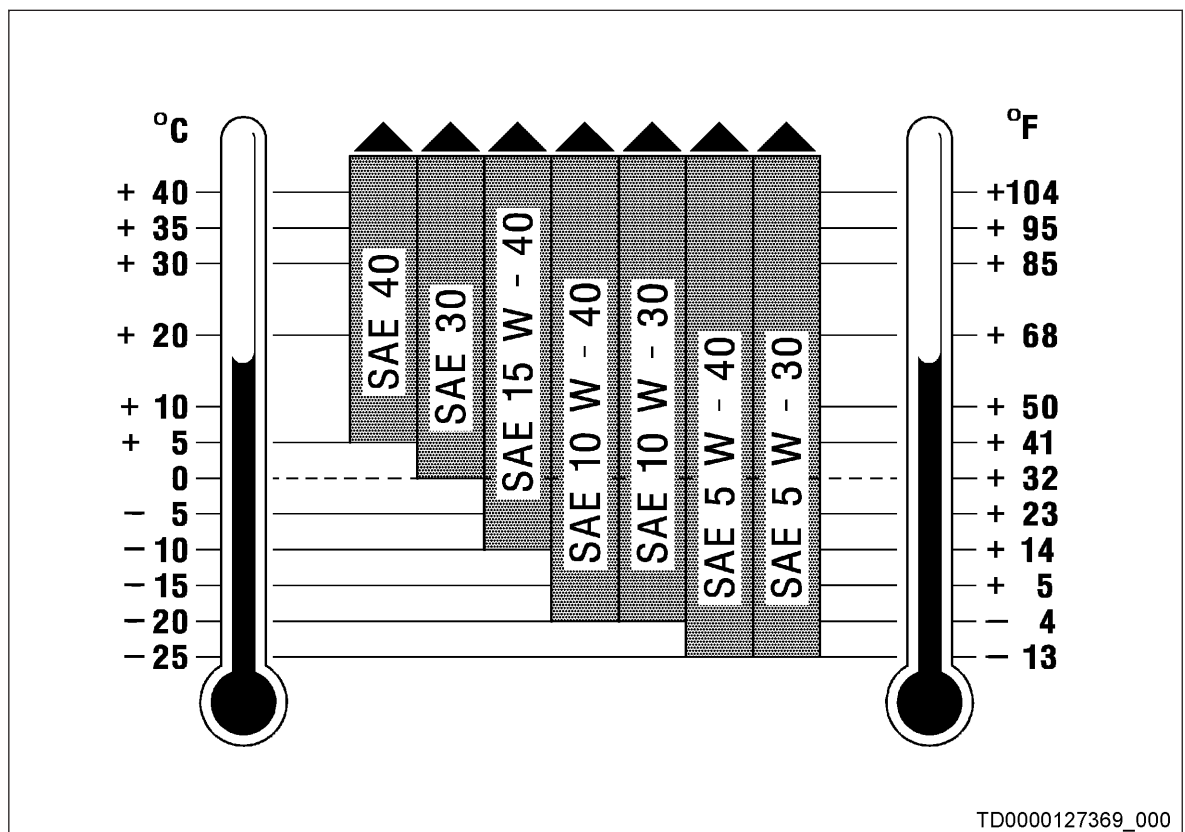
Figure 1: Relationship between the viscosity grades and the operating temperature ranges
