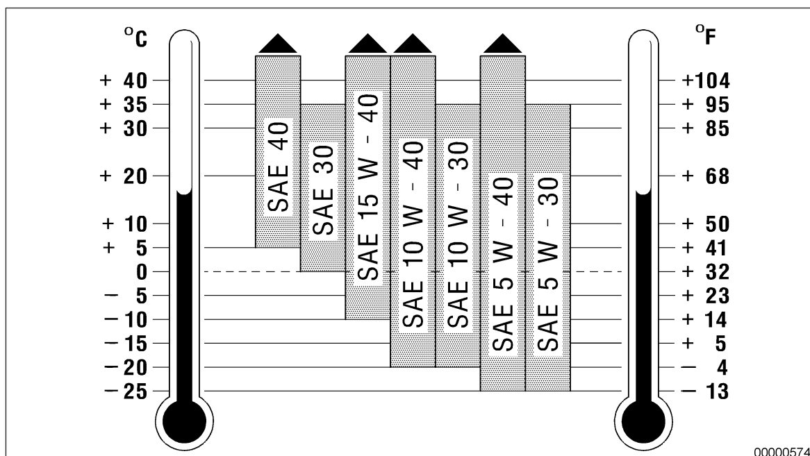
Figure 1: Relationship between viscosity grades and the operating temperature ranges
