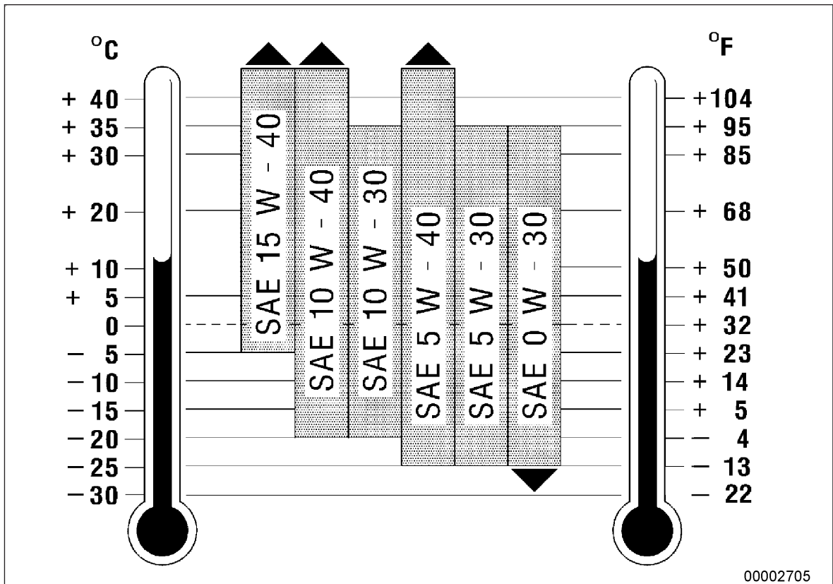
Figure 1: Viscosity grades
